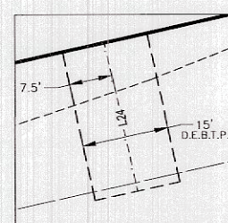
TYPICAL DRAINAGE EASEMENT
